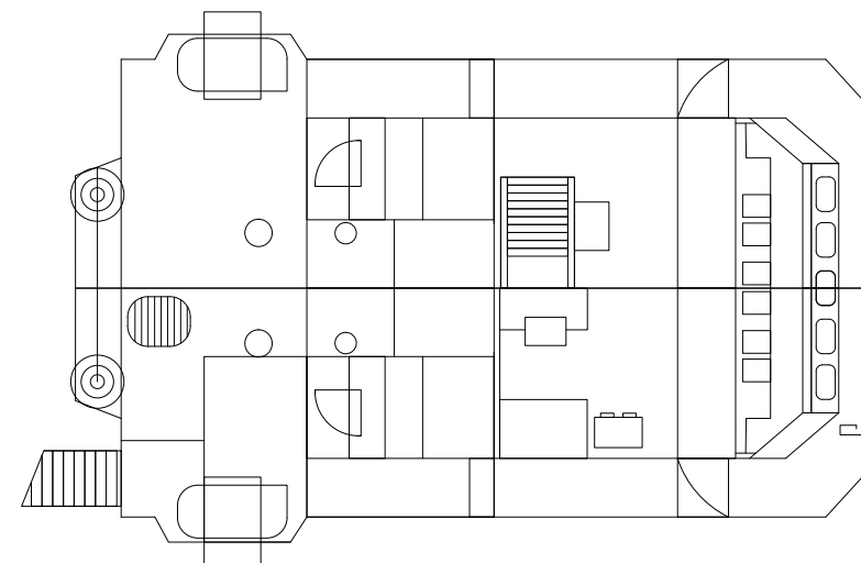
WHEELHOUSE DECK
